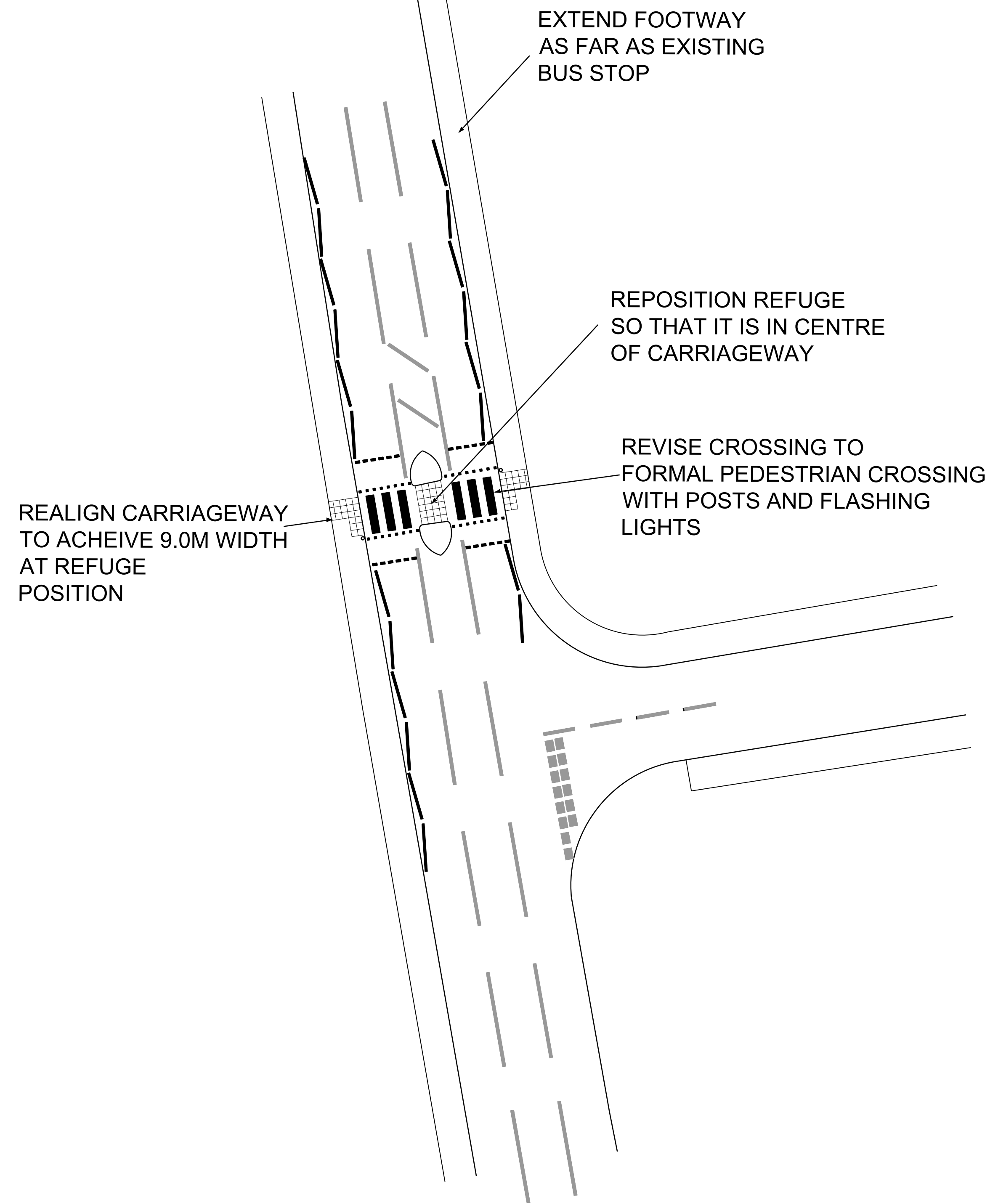
Proposed Layout Plan 1:200
