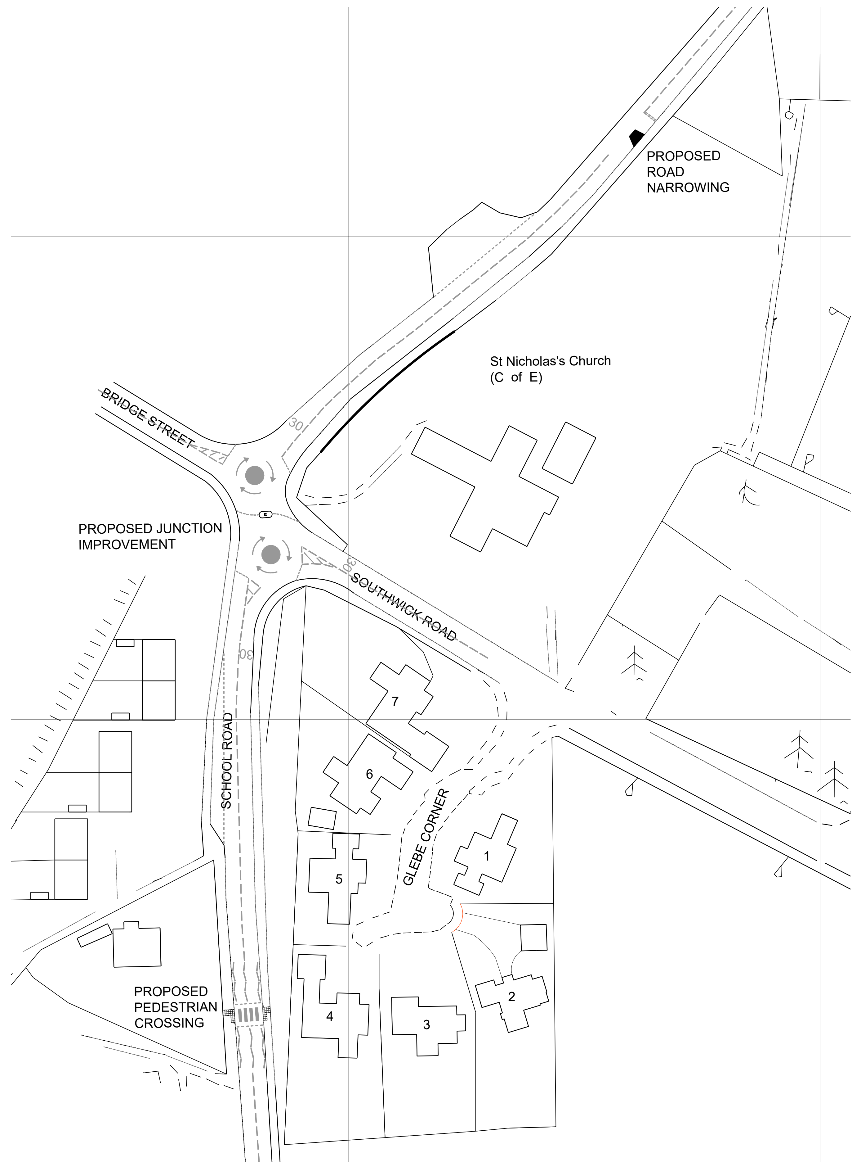
Proposed Layout Plan 1:500
